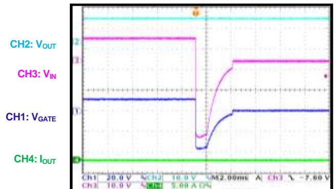
Negative Pulse
