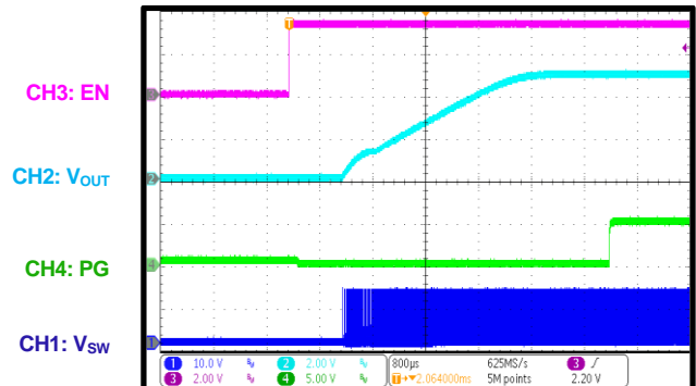
PG in Start-Up through EN
