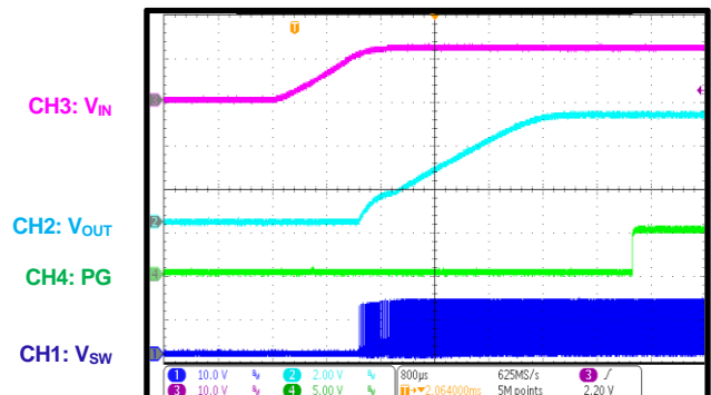
PG in Start-Up through VIN
