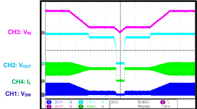
V IN Ramping Down and Up
