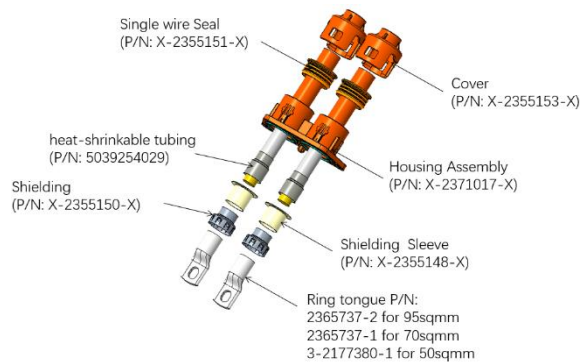
Figure 2: explosion view
