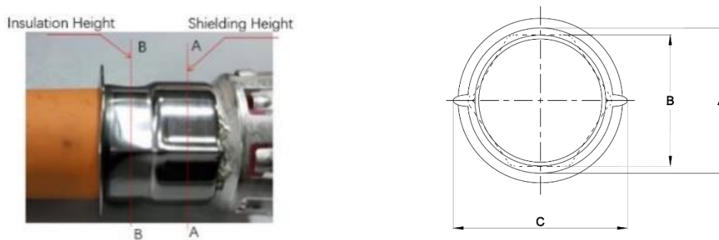
Figure 12: round crimp for shielding and hex crimp for insulation crimp
