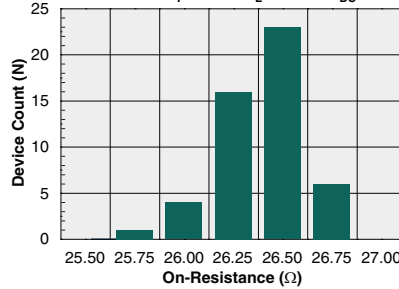
Typical On-Resistance Distribution (N=50, I_F=5mA , I_L=100mA_{DC} )
