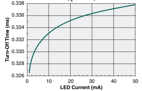
Typical Turn-Off Time vs. LED Forward Current ( I_L=60mA )
