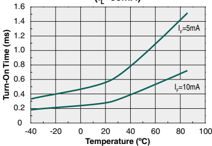
Typical Turn-On Time vs. Temperature ( I_L=60mA )
