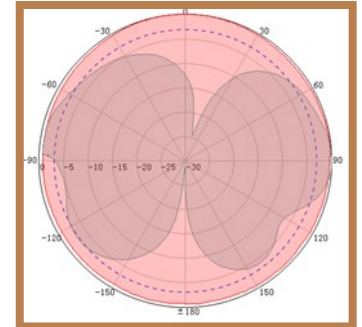
Antenna Radiation Pattern
