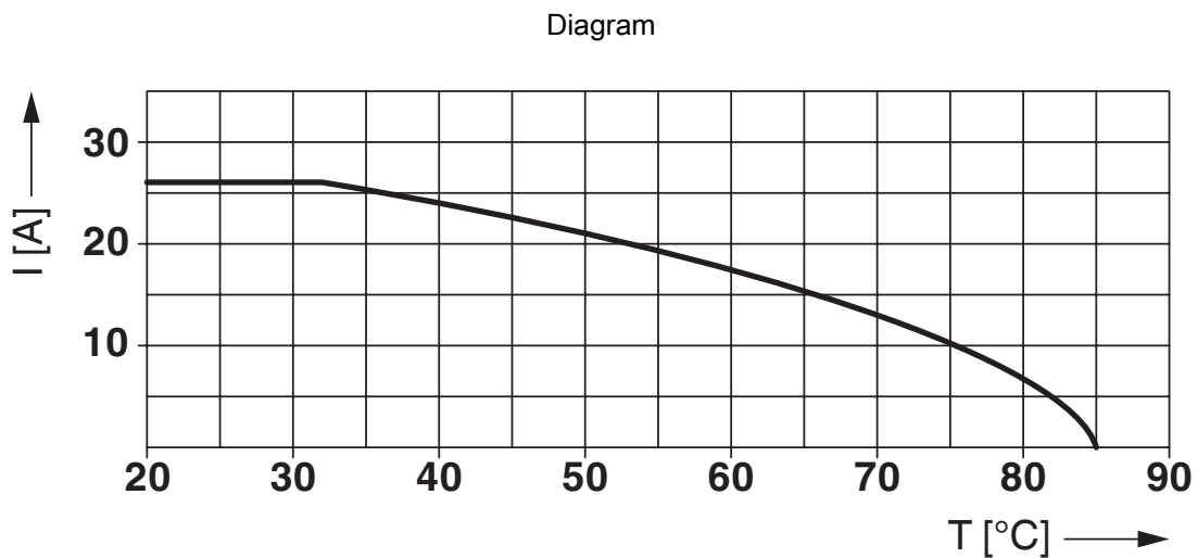
Nominal current depending on ambient temperature
