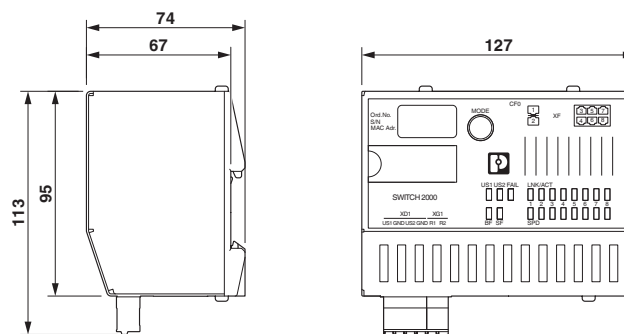
Dimensional drawing
